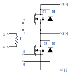
Half Bridge with Recovery Diode (3x6A)
