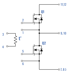
Half Bridge (6x6)
