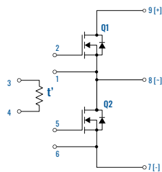
Half Bridge without Recovery Diode (3x6A)
